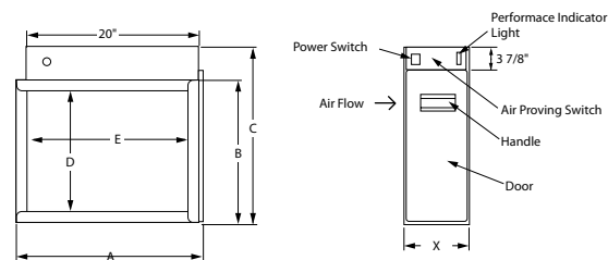
GA50A20, 22, 14 Dimensions
